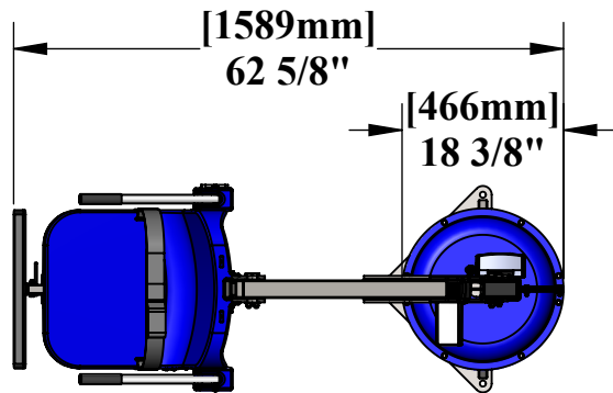
LOADING POSITION
