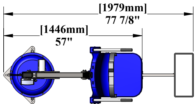
ABOVE WALL
