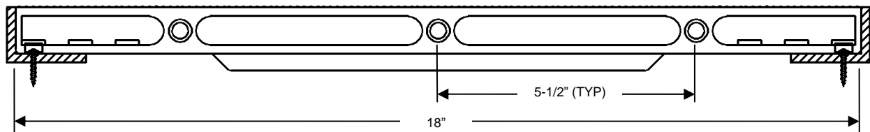
SIDE VIEW – 18"
