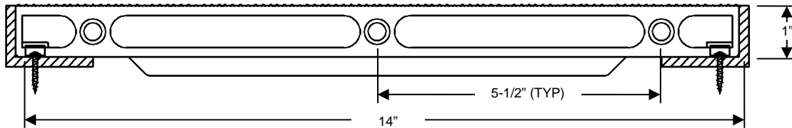
SIDE VIEW – 14"
