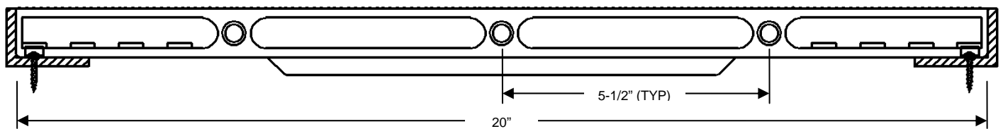
SIDE VIEW – 20"
