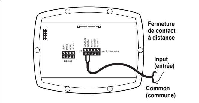
Figure 5. Raccordement aux contacts à distance
